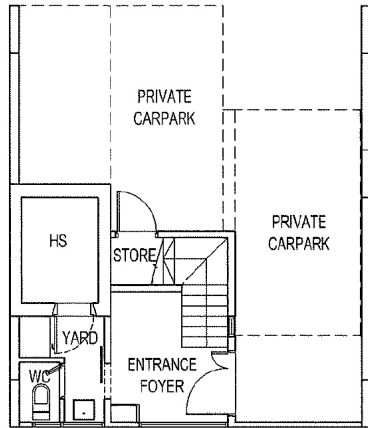
BASEMENT PLAN
